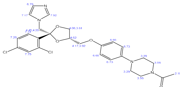
ChemNMR 1 H Estimation
